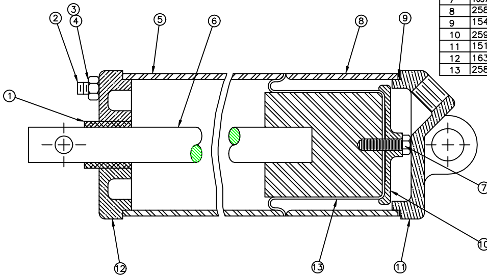
TIMING CYLINDER (No.21) (PART No. A-4091)
